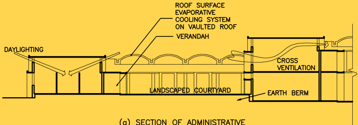
(a) SECTION OF ADMINISTRATIVE AND TECHNICAL BLOCK
