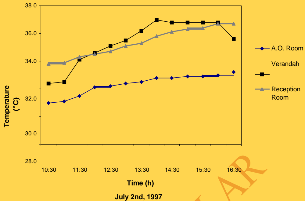
Fig. 7.9 Comparison of indoor temperatures - Solar Energy Centre, Gurgaon
