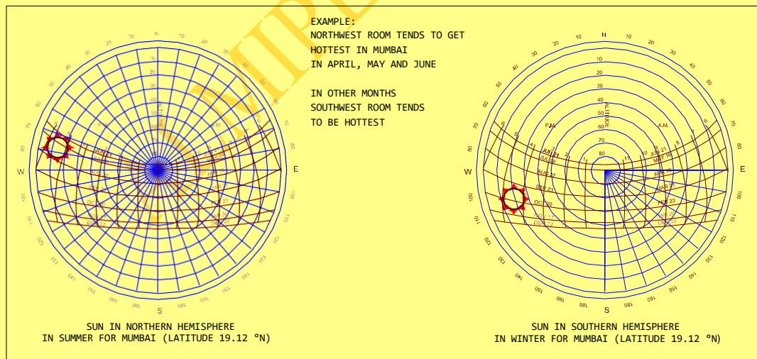
Fig. 2.1 Factors affecting solar radiation (a) effect of orientation, (b) effect of season
