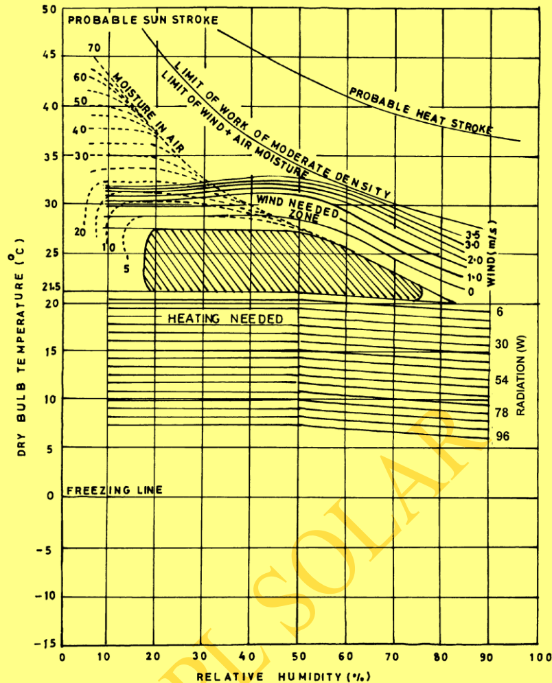
Fig. 2.14 Bio-climatic chart
