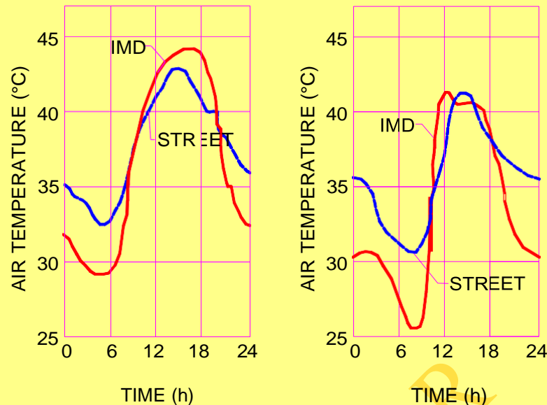
Fig. 2.16 Street temperatures in Jaisalmer [18] (a) Summer, (b) Winter
