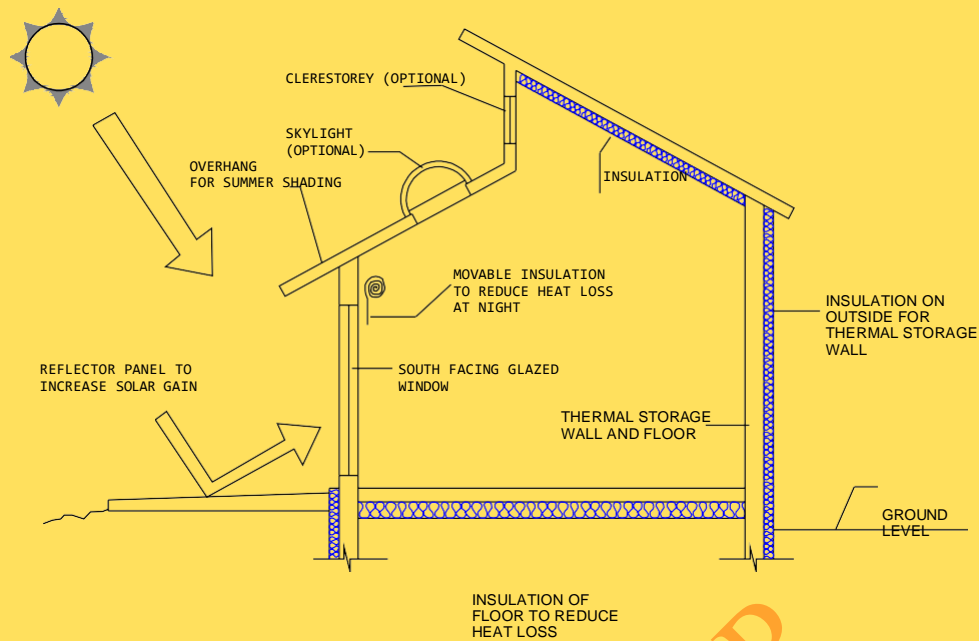
Fig. 3.12 Components of a direct gain system
