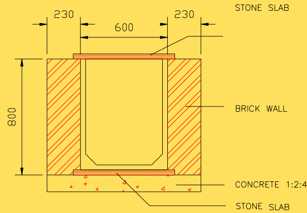
Fig. 3.35 Cross-section of pipe at the Dilwara Bagh House, Gurgaon
