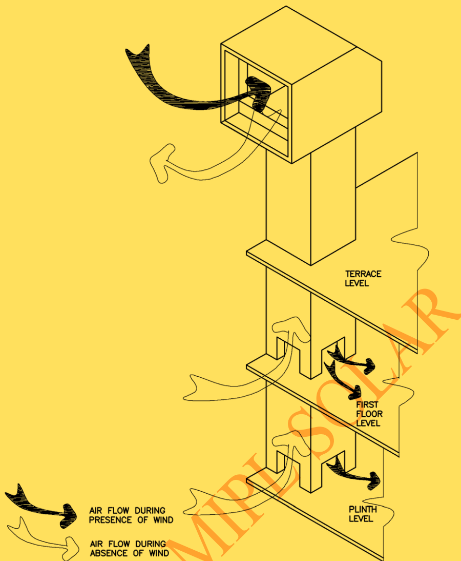
Fig. 3.25 Working principle of a wind tower
