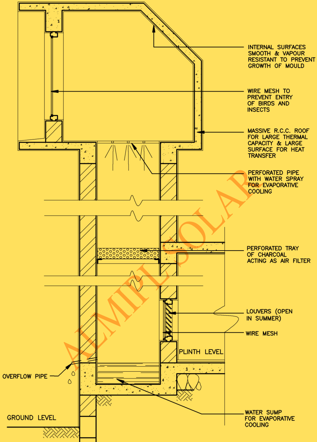
Fig. 3.26 Detail of a wind tower
