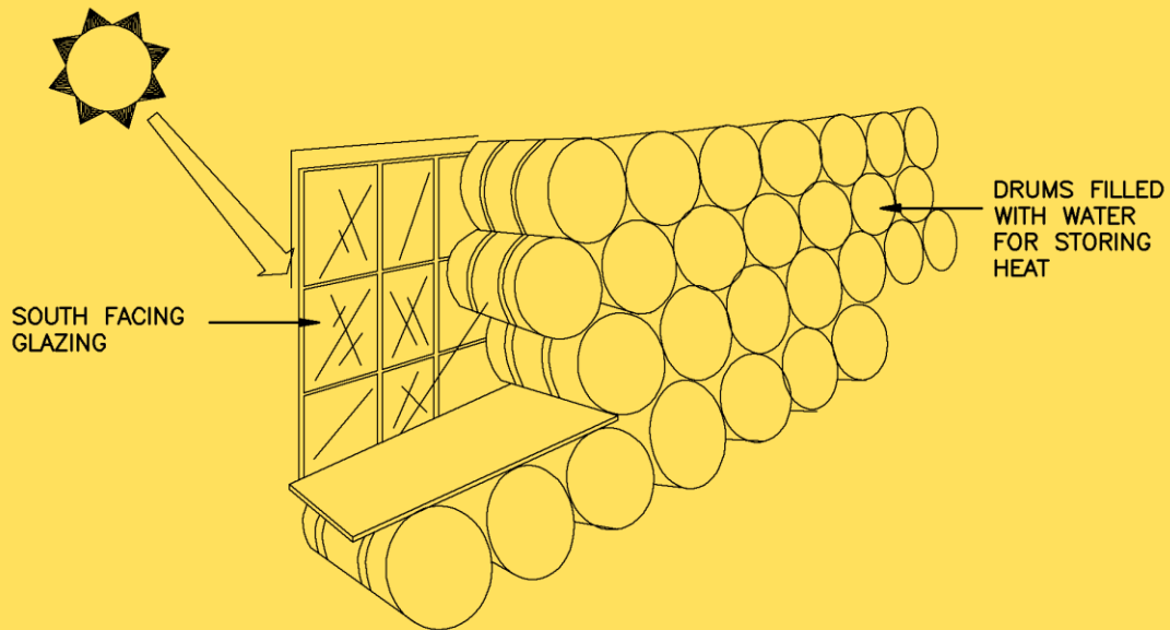
Fig. 3.16 Water wall
