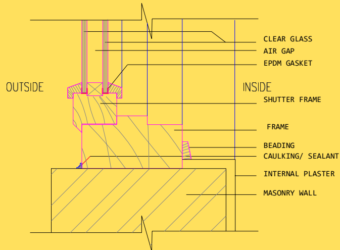
Fig. 3.13 Details of a double glazed window
