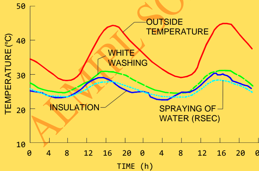
Fig. 3.7 Relative performance of different techniques on a flat roof [5]
