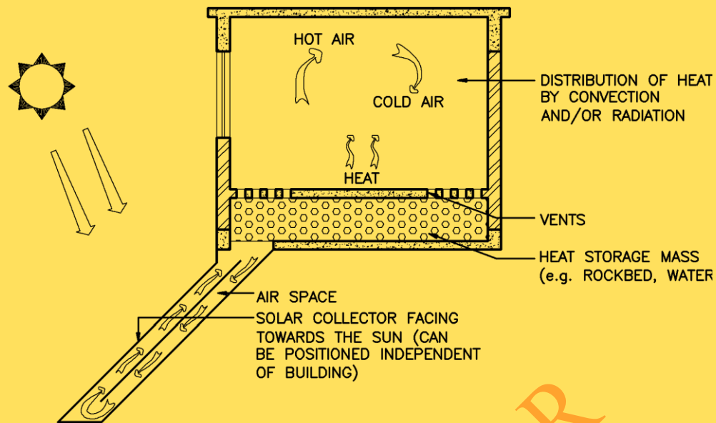
Fig. 3.22 Isolated gain
