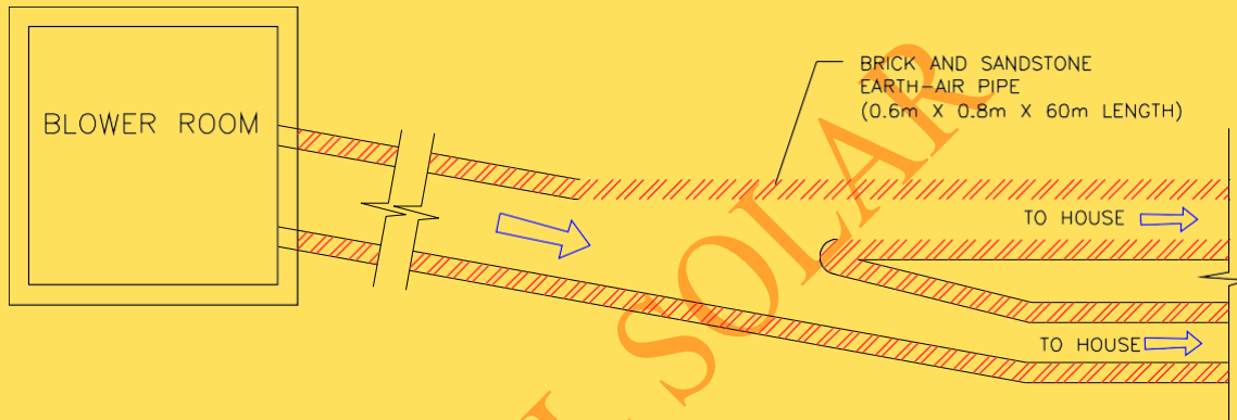
Fig. 3.36 Sketch plan of earth-air pipe system at the Dilwara Bagh House, Gurgaon
