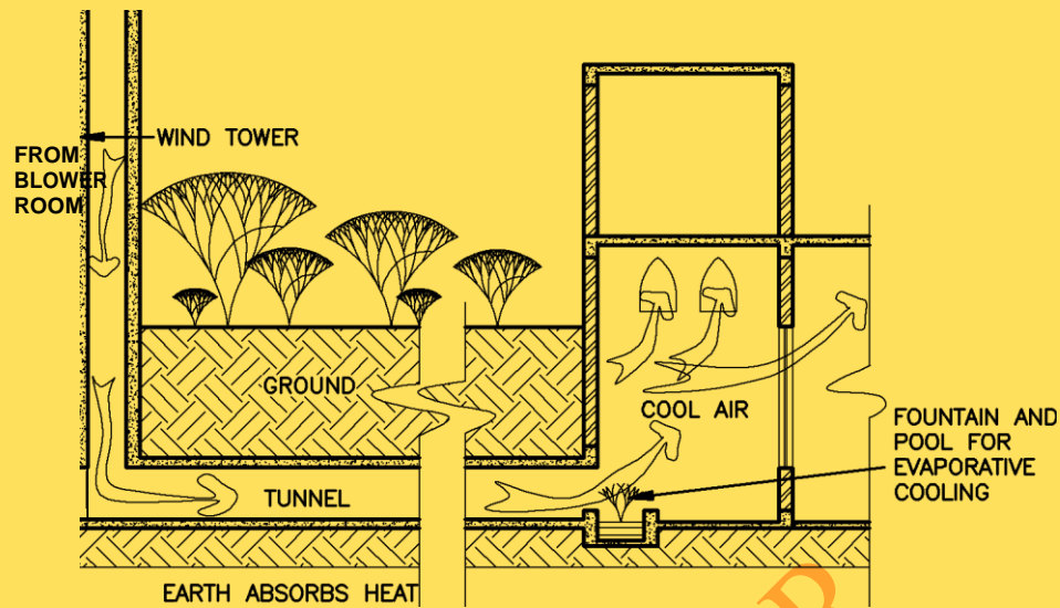
Fig. 3.34 Earth-air pipe system: working principle
