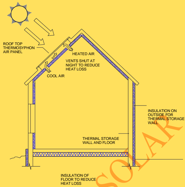
Fig. 3.18 Thermosyphon air panel: working principle
