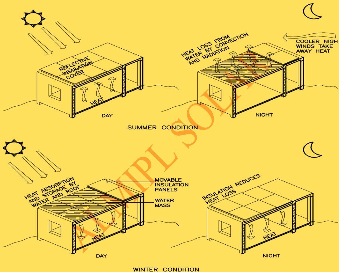
Fig. 3.31 Working principle of a roof pond
