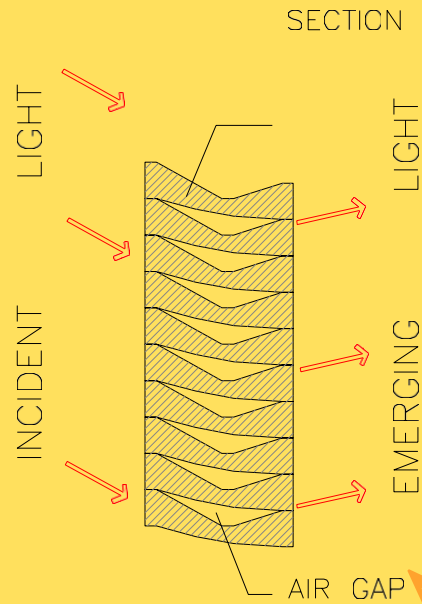
Fig. 3.48 Schematic sketch of a refractive daylighting device
